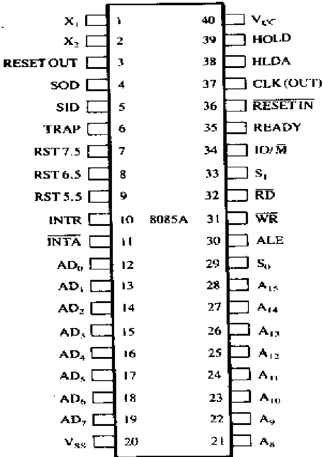
8085 Pinout
